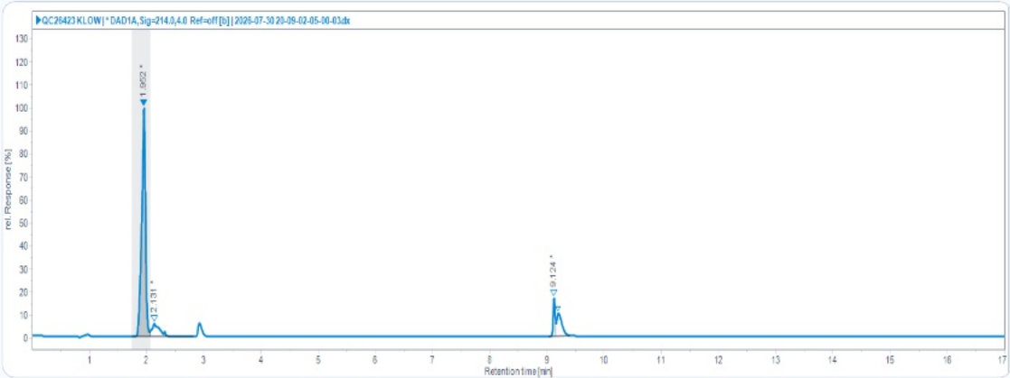
HPLC Chromatogram (Retention Time: 1.952, 2.131, 9.124, 9.202 min)
