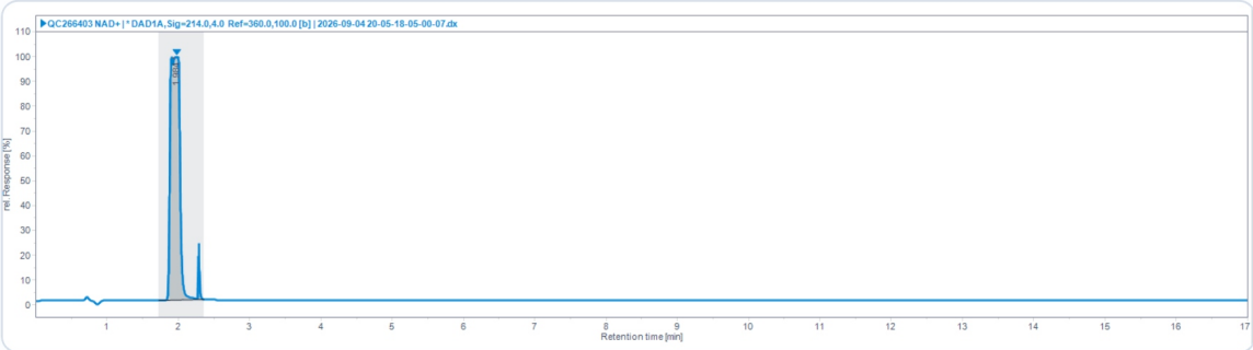
HPLC Chromatogram · Retention Time 1.984 min
